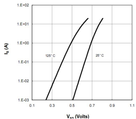
Figure 6: Body-Diode Characteristics
