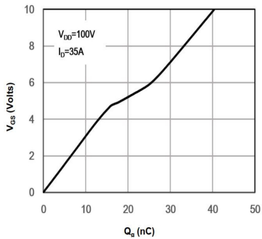
Figure 7: Gate-Charge Characteristics
